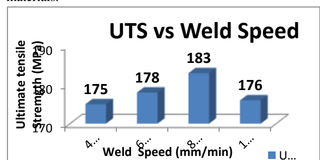
Fig.4: The effects of welding speed on ultimate tensile strength of the dissimilar joints
